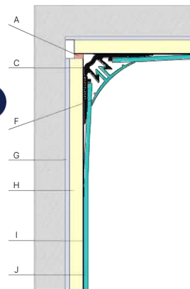
FIN'ANGLE ALU
