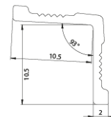
FIN'ANGLE ALU
